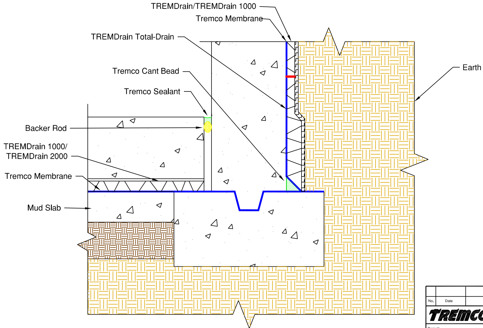
Typical Below-Grade Detail w/Drainage
